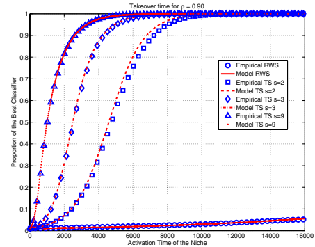
Figure 2: Empirical and the theoretical takeover time for roulette wheel selection and tournament selection with s=2 , s=3 and s=9 when (a) \rho = 0.50 and (b) \rho = 0.90 .
