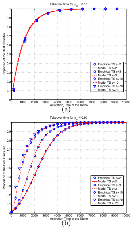
Figure 6: Takeover time for tournament selection when (a) \rho_m is 0.1 and (b) \rho_m is 0.9.
