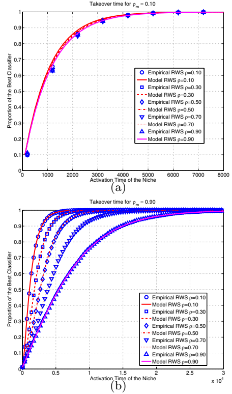
Figure 5: Takeover time for roulette wheel selection when (a) \rho_m is 0.1 and (b) \rho_m is 0.9.
