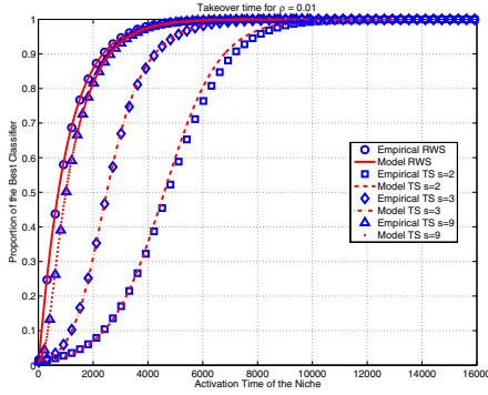
Figure 1: Empirical and the theoretical takeover time when \rho = 0.01 for roulette wheel selection and tournament selection with s=2 , s=3 and s=9 .
